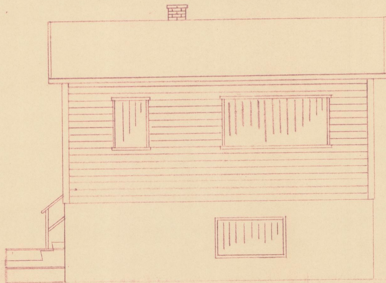
Fasade Vest.
